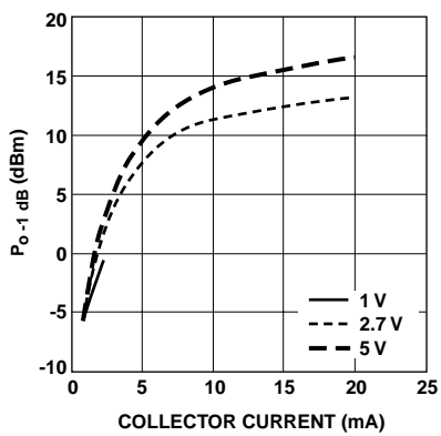
Figure 7. AT-32032 P_{1\text{ dB}} vs. Collector Current and Voltage (valid up to 2.4GHz).
