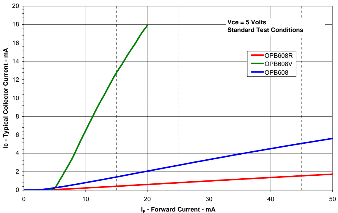
Collector Current vs Diode Forward Current
