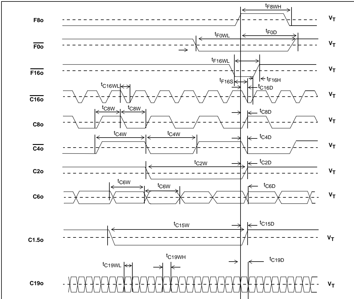
Figure 12 - Output Timing 1
