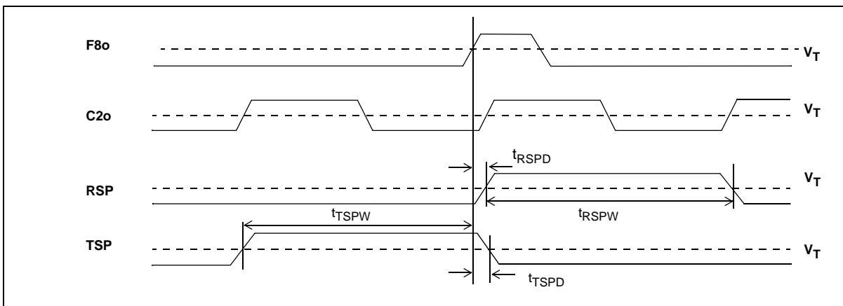
Figure 13 - Output Timing 2
