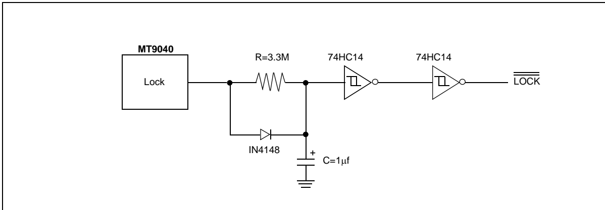
Figure 8 - Time-constant Circuit
