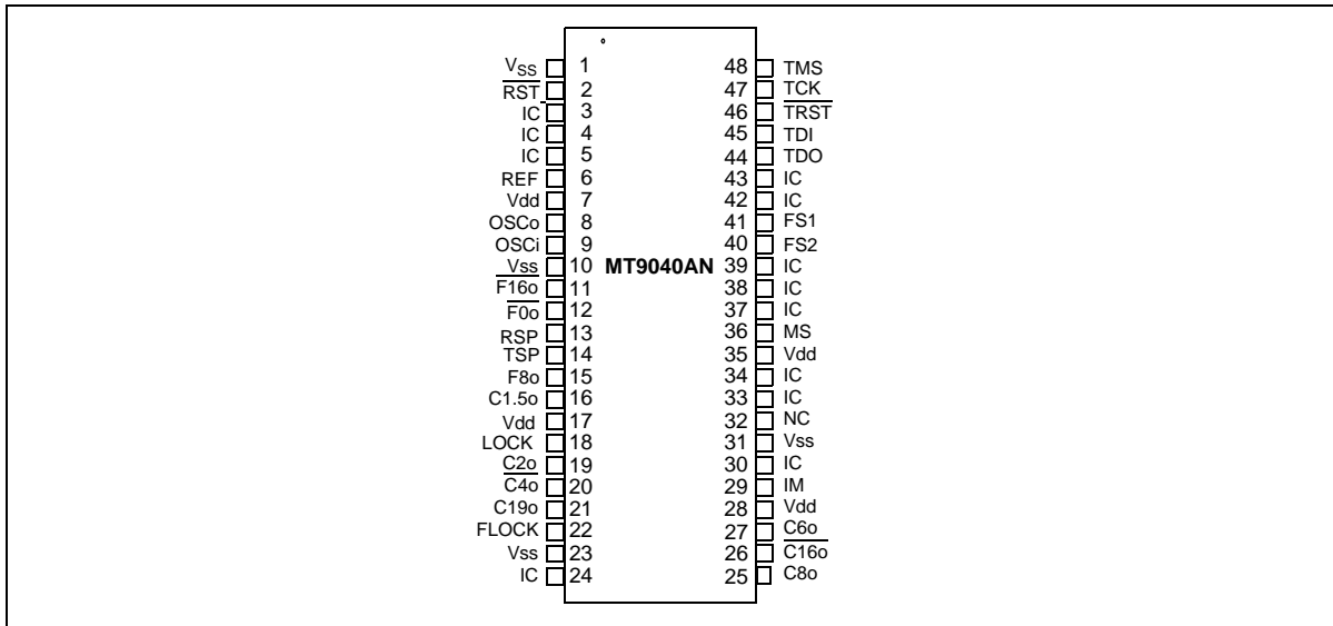
Figure 2 - Pin Connections
