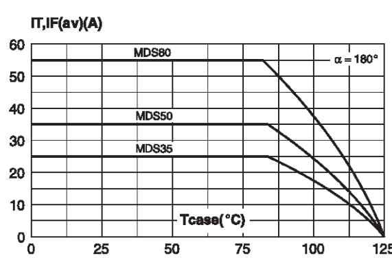
Fig. 2-1: Average on-state current versus case temperature (thyristor or diode, sinusoidal waveform).
