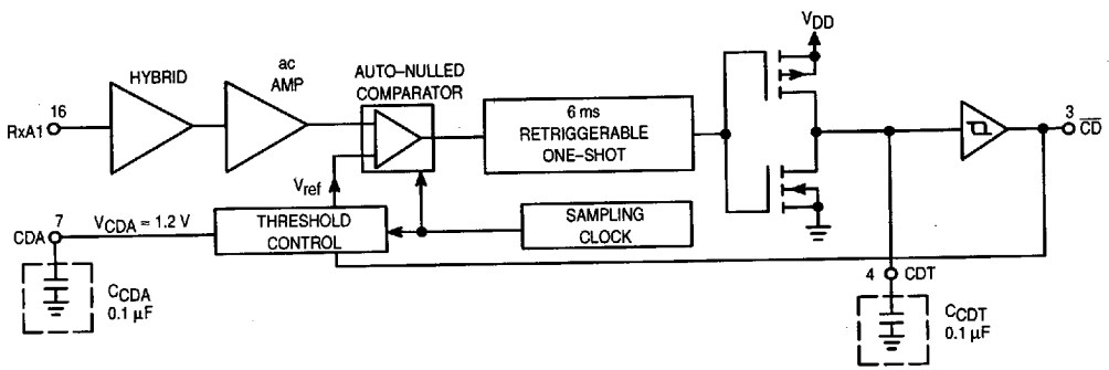
Figure 5. Carrier Detect Circuit
